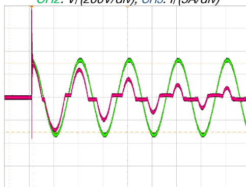
Figure 3 - Inrush current, V_i = 230\text{Vac} , 90^\circ CH2: V_i (200V/div), CH3: I_i (5A/div)
