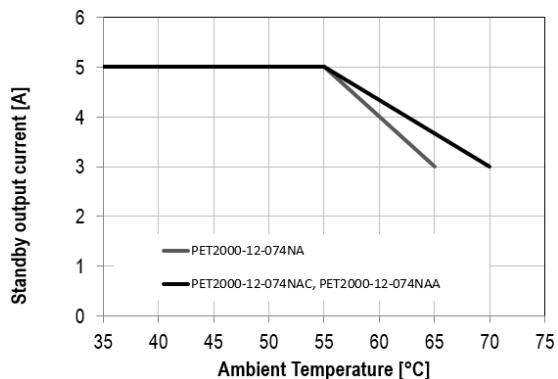
Figure 40 – Maximum ISB
