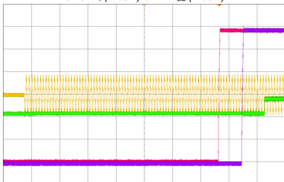
Figure 4 - Turn-On AC Line 230VAC, full load (200ms/div)
