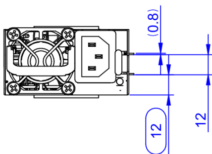
Figure 43 – Front View
