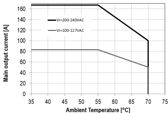
Figure 38 – Maximum I_I PET2000-12-074NAA (Anderson Saf-D-Grid®)
