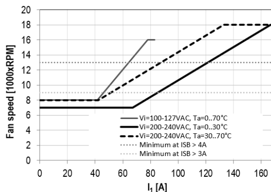
Figure 33 - Fan speed vs. main output load
