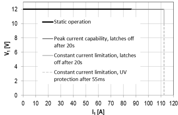
Figure 14 - Current Limitation on V_I at V_I = 90 \dots 140\text{VAC}
