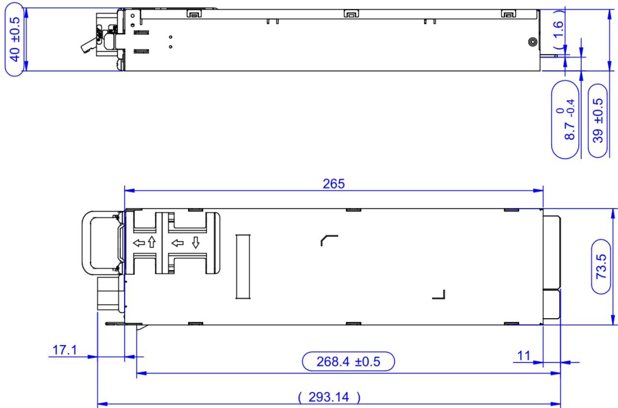
Figure 45 – Top and side view
