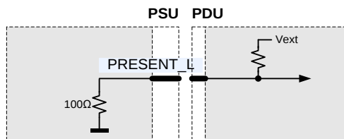
Figure 22 – PRESENT_L connection
