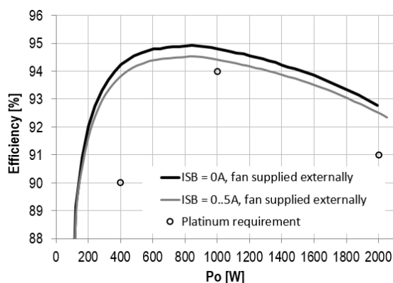
Figure 1 - Efficiency vs. Load current, V_i = 230\text{VAC} (ratio metric loading)
