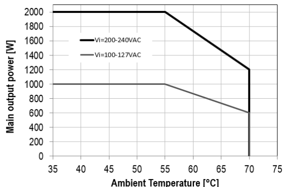
Figure 39 – Maximum P_I PET2000-12-074NAA (Anderson Saf-D-Grid®)
