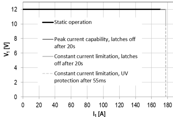
Figure 15 - Current Limitation on V_I at V_I = 180 \dots 264\text{VAC}
