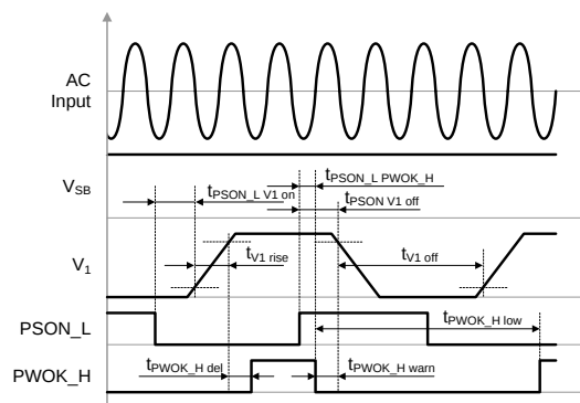
Figure 26 - PS_ON_L turn-on/off timing
