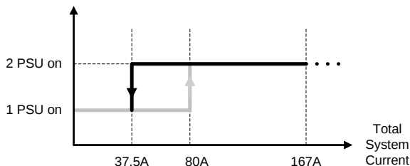
Figure 19 - Hot-standby enable/disable current thresholds
