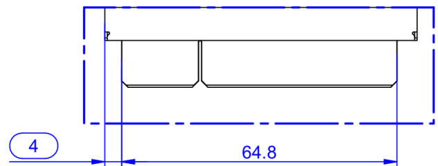
Figure 47 – Detail A
