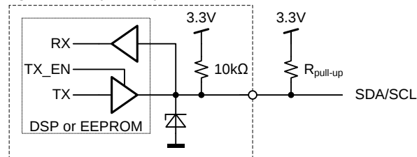
Figure 27 - Physical layer of communication interface
