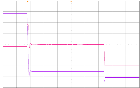
Figure 11 - Load transient V_I , 167 to 83A (500 \mu s/div)
