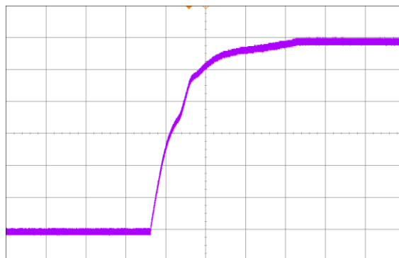
Figure 5 - Rise time V_i at 230VAC, full load (2ms/div)
