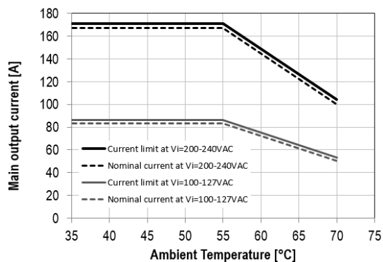
Figure 41 – Current limitation vs temperature
