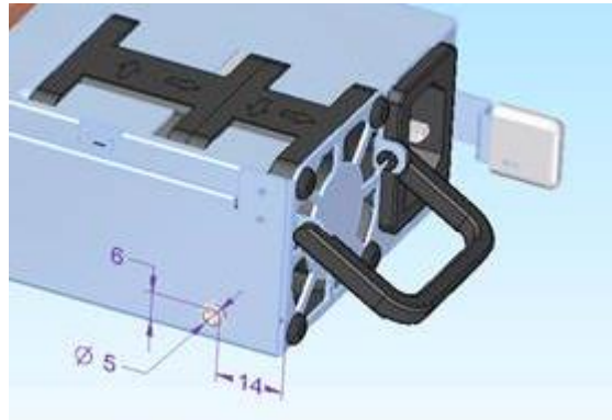
Figure 48 – Polarizing screw
