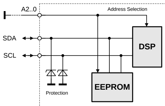
Figure 30 - I 2 C Bus to DSP and EEPROM
