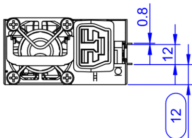
Figure 46 – Front view
