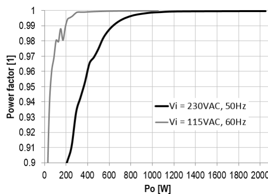
Figure 2- Power factor vs. Load current
