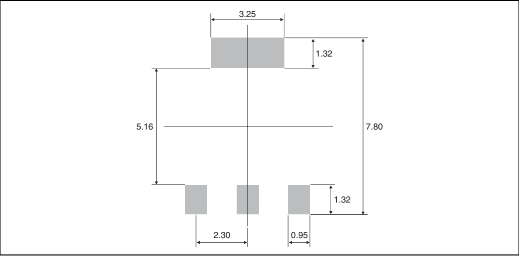
Figure 15. SOT-223 footprint dimensions (in millimeters)
