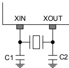
Figure 7.8 Crystal/Ceramic Oscillator
