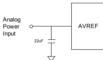
Figure 11.32 A/D Power (AVDD) Pin with Capacitor
