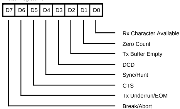
Read Register 0
