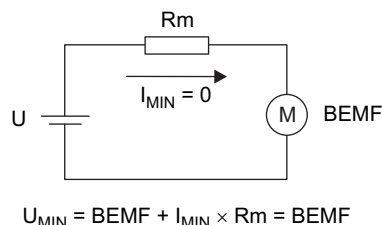
Figure 32. Mechanical AVS
