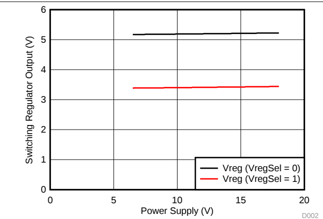
Figure 2. Switching Regulator Output vs Power Supply
