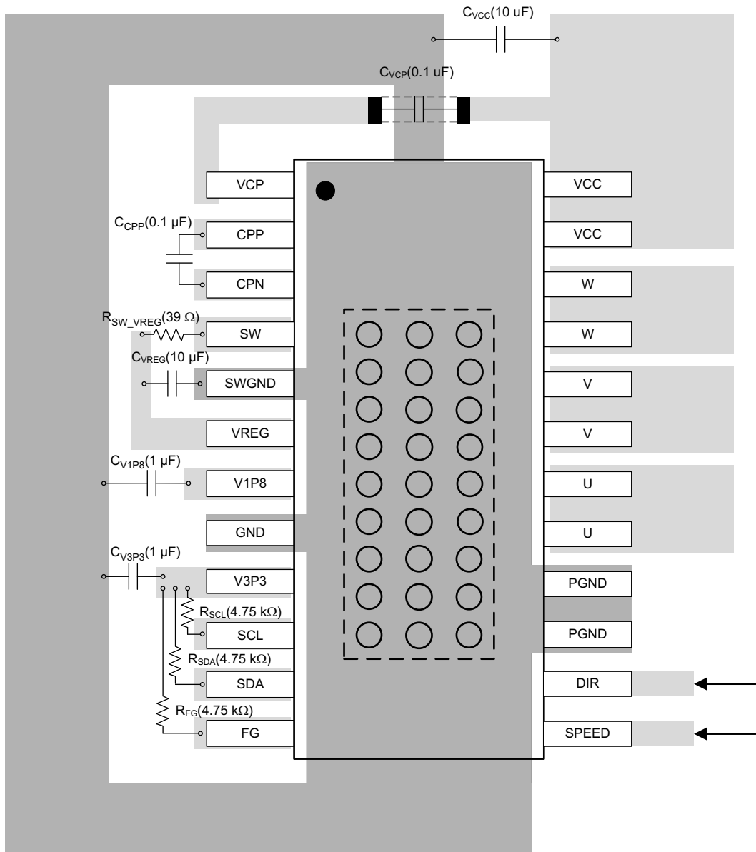
Figure 42. Layout Schematic
