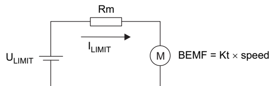
Figure 25. Acceleration Current Limit
