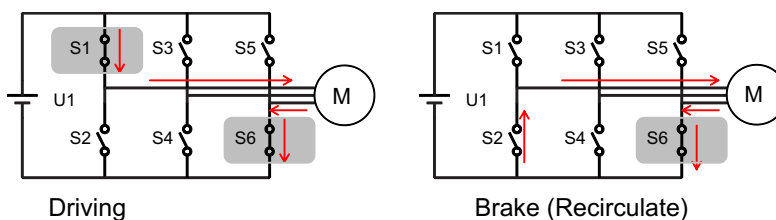
Figure 13. IPD Release Mode 0
