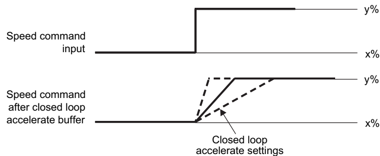
Figure 23. Closed-Loop Accelerate
