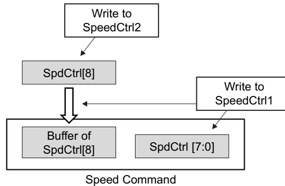
Figure 22. I²C Mode Speed Control
