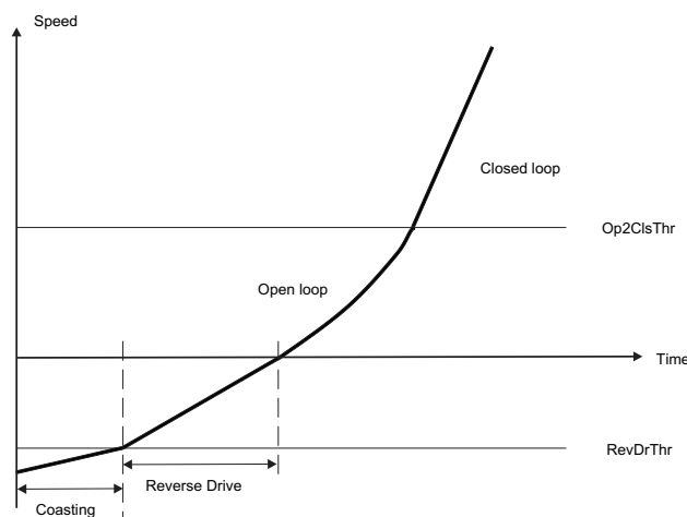
Figure 11. Reverse Drive Function
