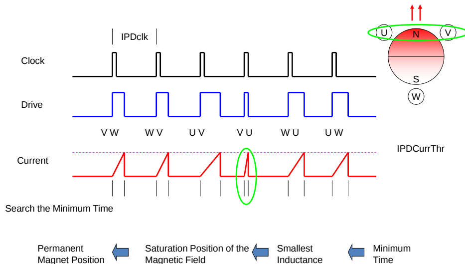
Figure 12. IPD Function
