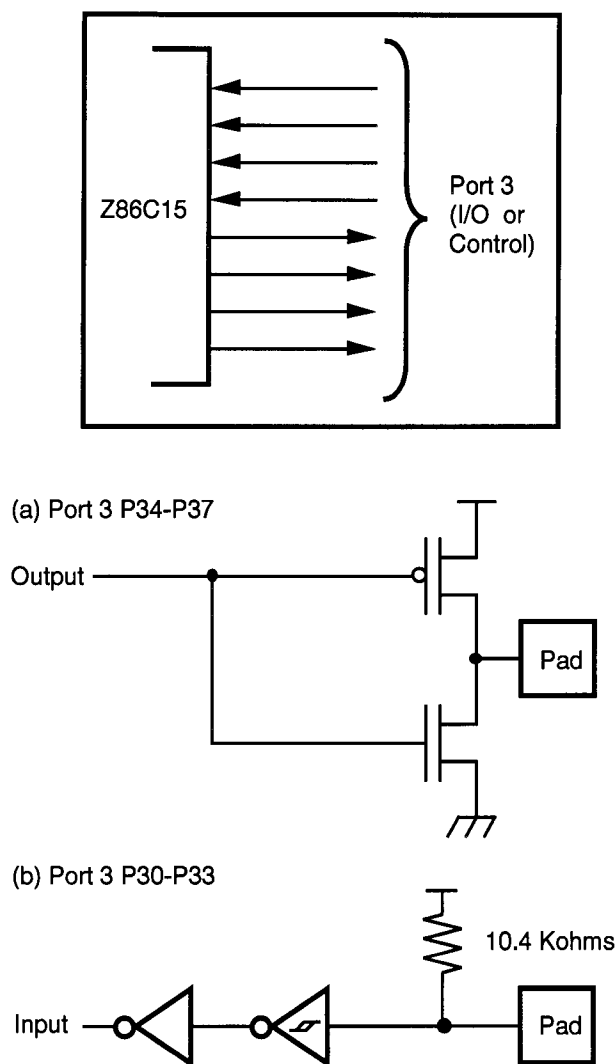
Figure 10. Port 3 Configuration
