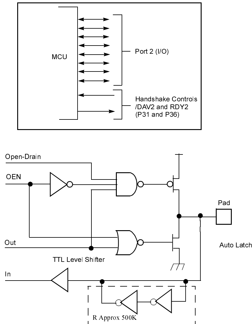
Figure 7. Port 2 Configuration
