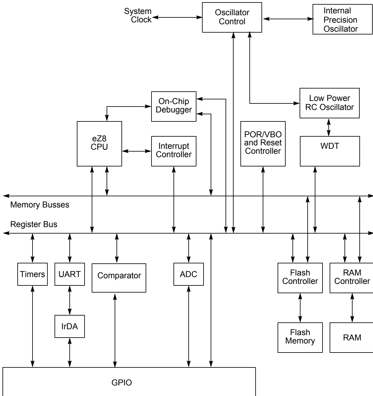
Figure 1. Z8 Encore! XP Z8F0823 Series Block Diagram
