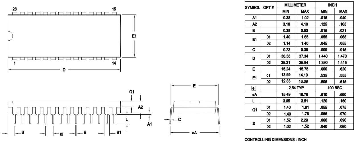
Figure 40 displays the 28-pin Plastic Dual Inline Package (PDIP) available for Z8 Encore! XP Z8F0823 Series devices.
