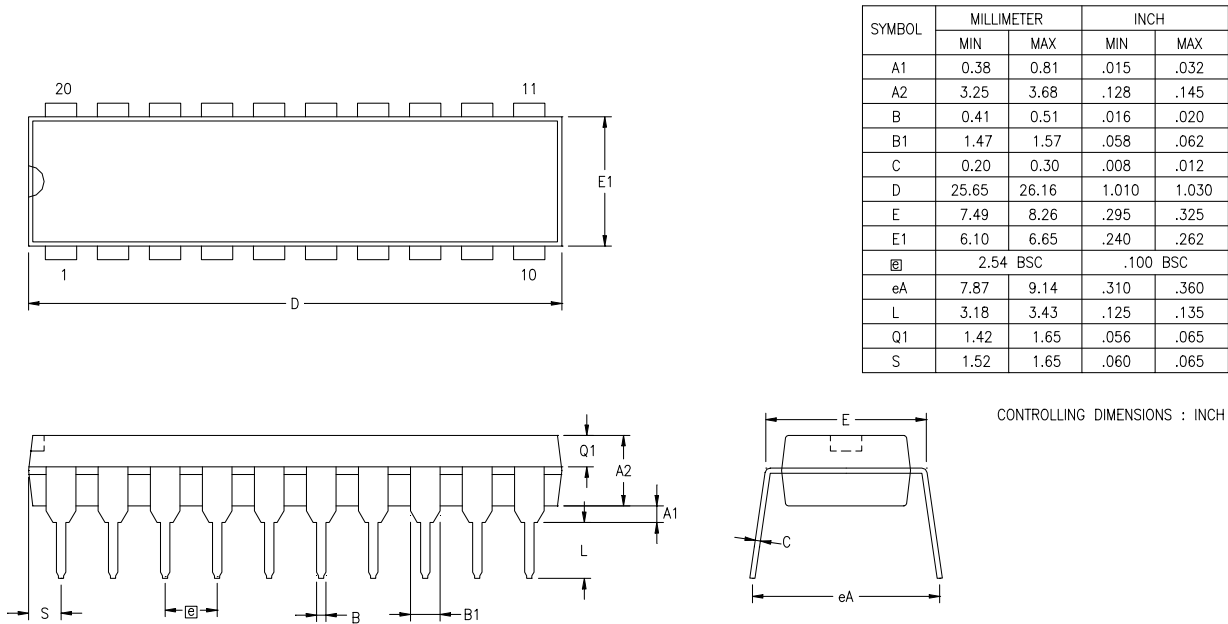
Figure 42 illustrates the 20-pin Plastic Dual Inline Package (PDIP) available for the Z8 Encore! XP 8K and 4K Series devices.
