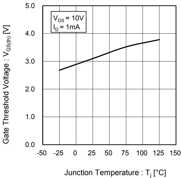
Fig.8 Gate Threshold Voltage vs. Channel Temperature
