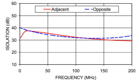
1. Total Loss = Insertion Loss + 13.8dB splitter loss. ZFSC-24-11-75 ISOLATION
