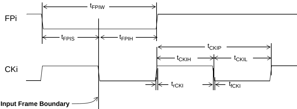
Figure 25 - Frame Pulse Input and Clock Input Timing Diagram (ST-BUS)
