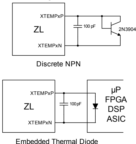
FIGURE 10. EXTERNAL TEMPERATURE MONITORING
