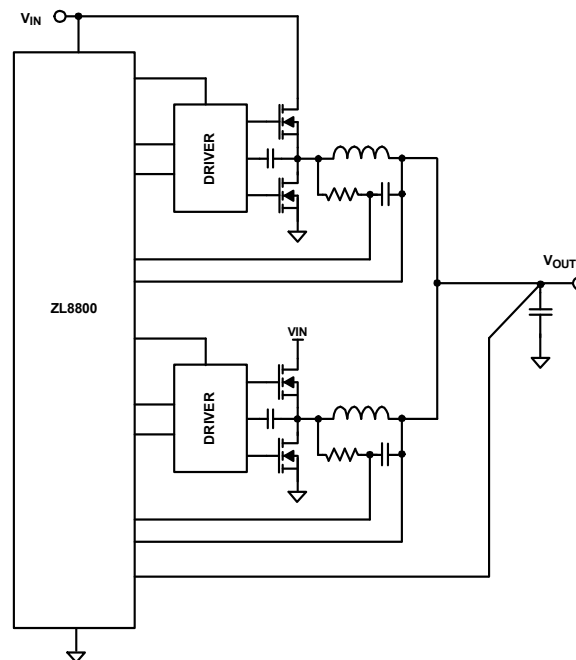
FIGURE 9. DUAL PHASE EXAMPLE
