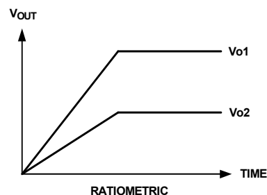
FIGURE 8. TRACKING MODES
