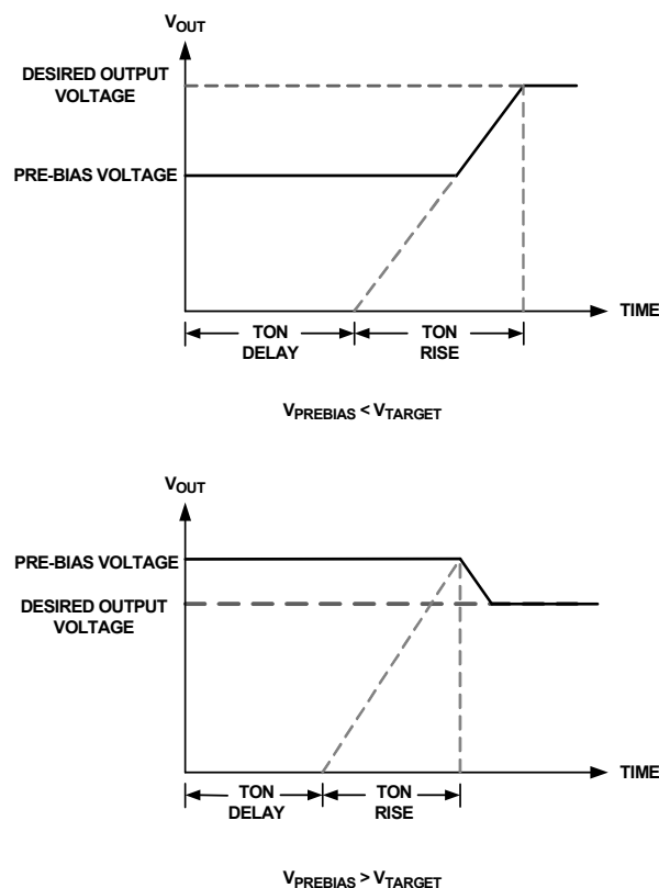
FIGURE 6. OUTPUT RESPONSES TO PREBIAS VOLTAGES
