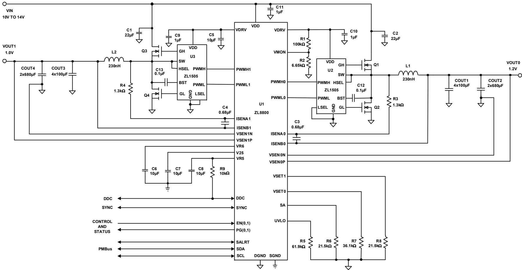
FIGURE 3. SCHEMATIC
