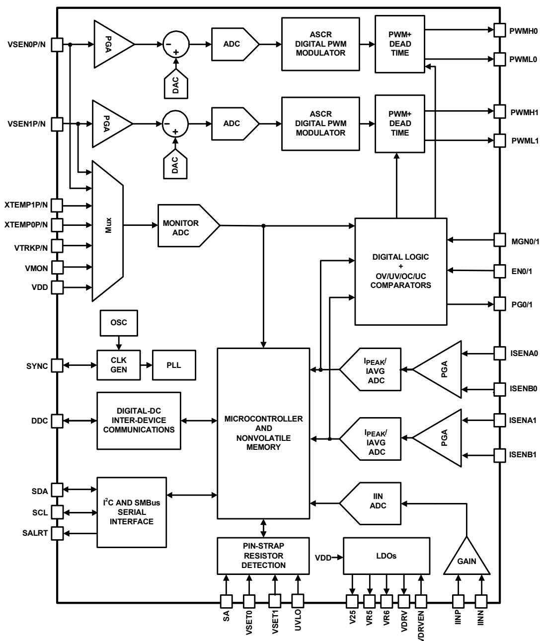
FIGURE 2. BLOCK DIAGRAM
