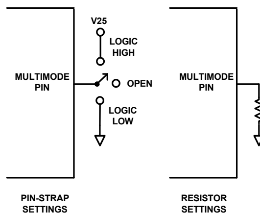
FIGURE 4. PIN-STRAP AND RESISTOR SETTINGS
