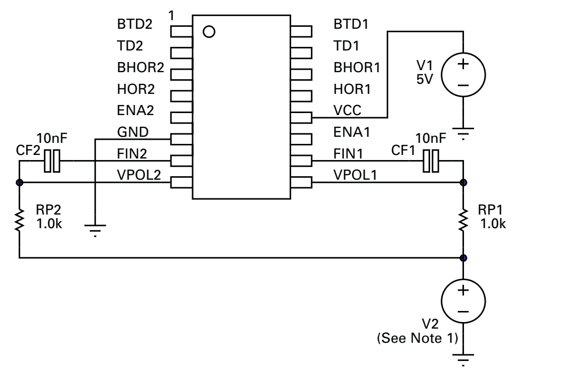
TEST CIRCUIT 1 (ZLNB2012 Pinout for QSOP16 package designator - Q16)
