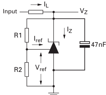
Fig 2 - Test circuit for V_Z > V_{ref}
