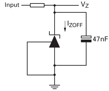
Fig 3 - Test circuit for Off state current †
