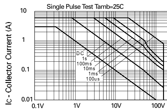
V_{CE} - Collector Voltage
