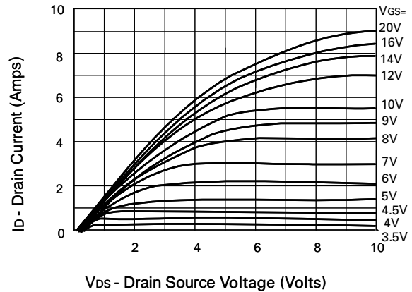
Saturation Characteristics
