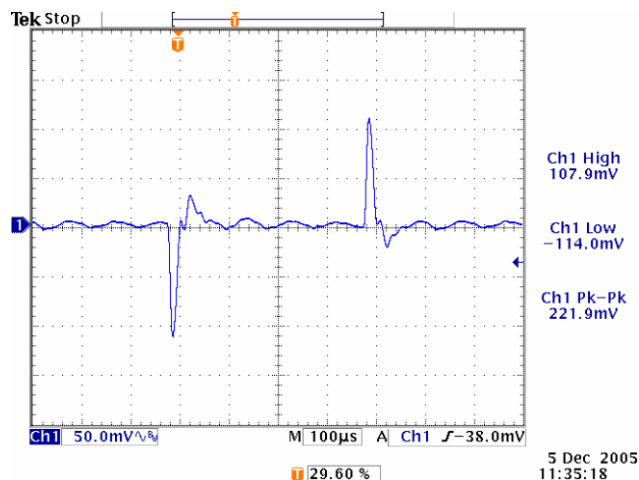
Figure 13. Vin=5V, Vout=2.5V. CCA=03
