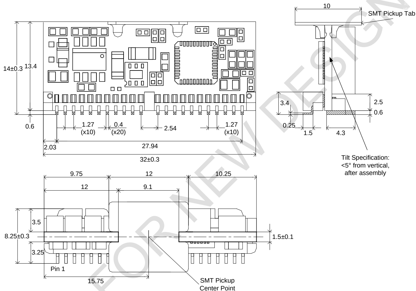
Figure 20. Mechanical Drawing
