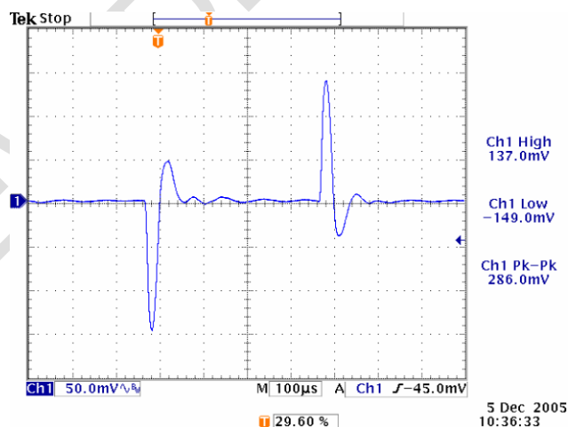
Figure 14. Vin=3V, Vout=1V. CCA=03
