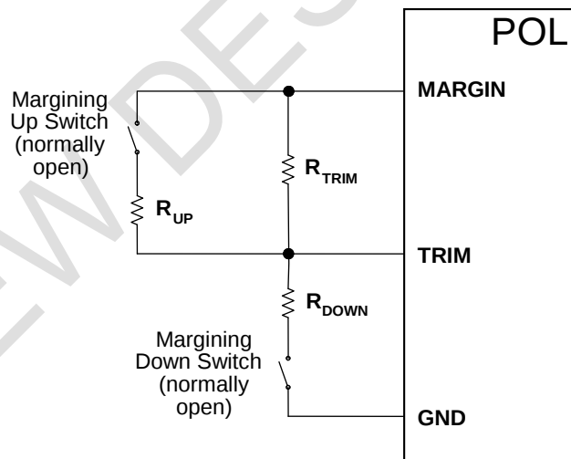
Figure 13. Alternative Margining Configuration
