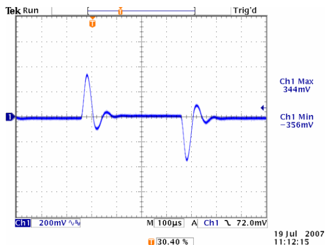
Figure 9. Vin=12V, Vout=2.5V. CCA=0
