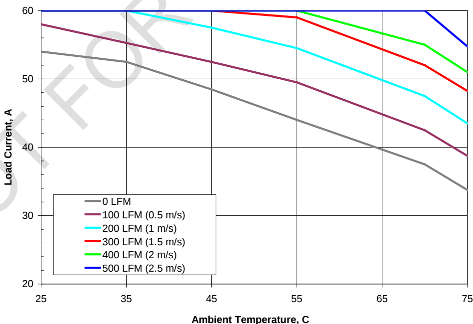
Figure 10. Thermal Derating Curves. Vin=12V, Vout=2.5V
