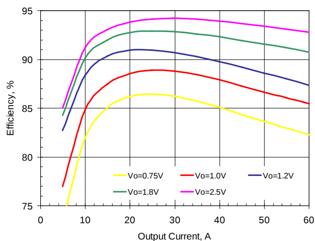
Figure 3. Efficiency vs. Load. Vin=12V
