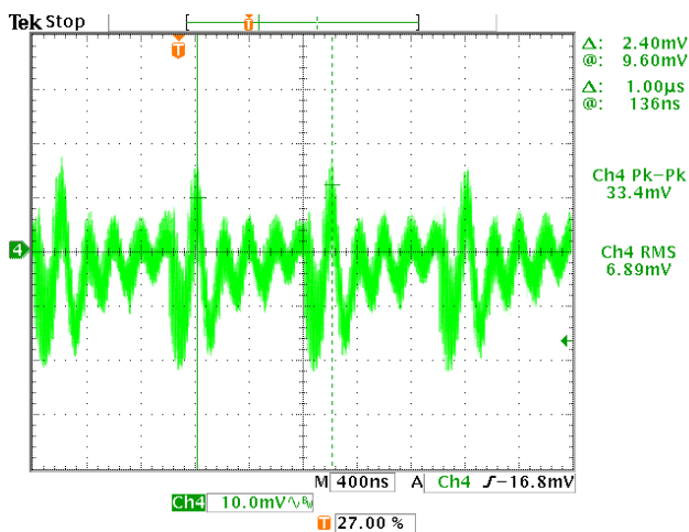
Figure 51. Input Voltage Noise with Interleave
