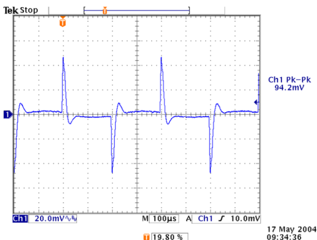
Figure 31. Transient Response without Optimal Voltage Positioning
