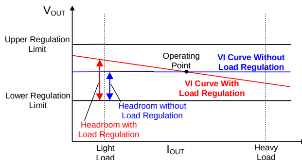
Figure 30. Concept of Optimal Voltage Positioning
