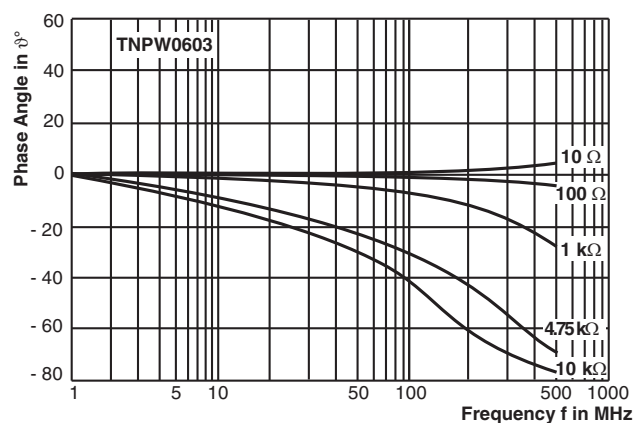
HF Performance
