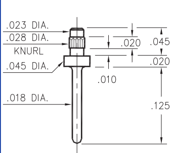
3157-0-00-XX-00-00-03-0 Press-fit in .026 mounting hole
