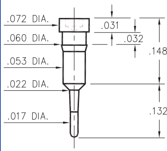
0915-0-00-XX-00-00-03-0 Press-fit in .057 mounting hole
