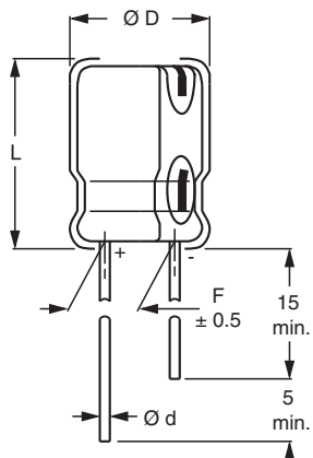
Fig.2 Form CA: Long leads
