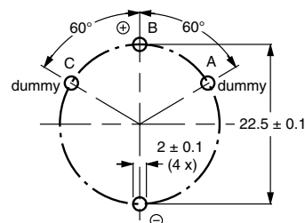
Fig.7 Mounting hole diagram
