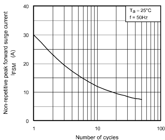
Fig. 10.5 Surge current
