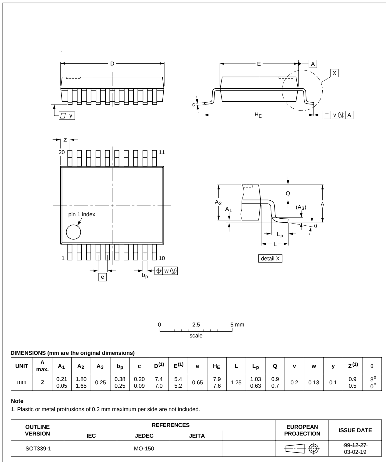
Fig 10. Package outline SOT339-1 (SSOP20)
