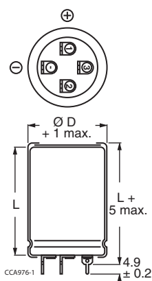
Case Ø D = 35 mm
