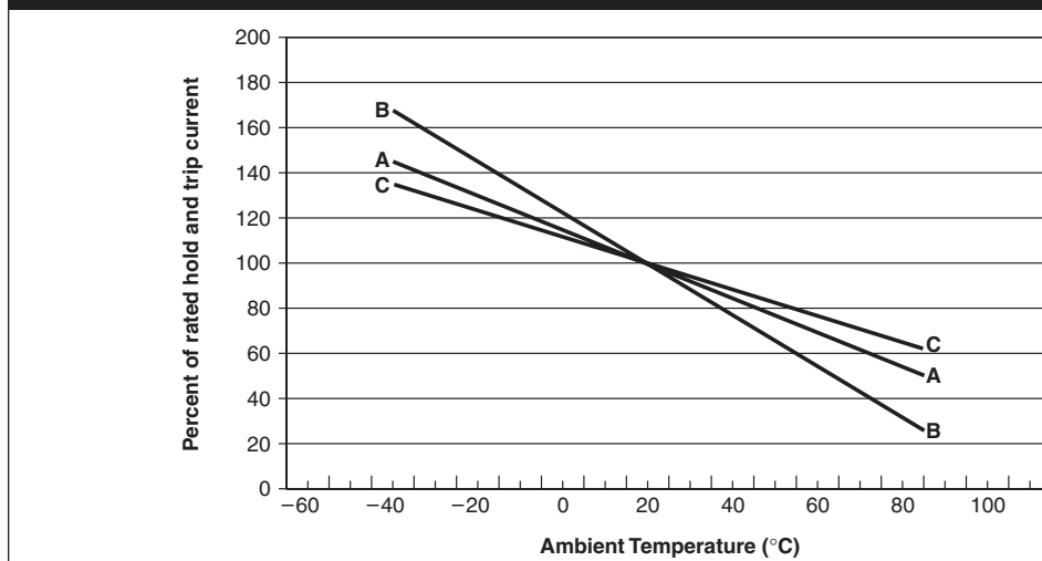
Figure S1. Thermal Derating Curve
