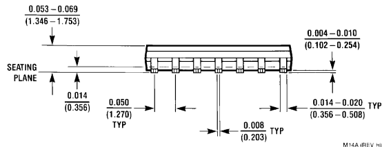
14-Lead Small Outline Package JEDEC (M) Order Number 74LCX08M or 74LCX08MX NS Package Number M14A
