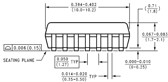
14-Lead Small Outline Package EIAJ (SJ) Order Number 74LCX08SJ or 74LCX08SJX NS Package Number M14D
