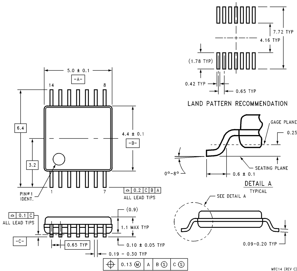
14-Lead Thin Shrink Small Outline Package, JEDEC Order Number 74LCX08MTC or 74LCX08MTCX NS Package Number MTC14
