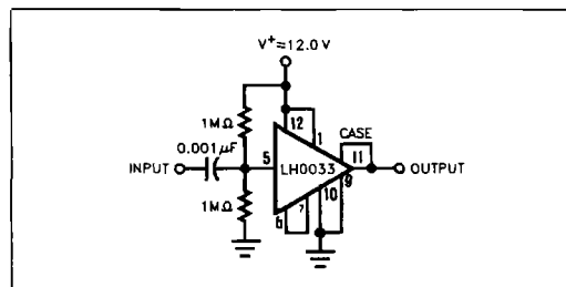
Figure 11. Single Supply AC Amplifier
