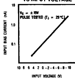
LH0033 INPUT BIAS CURRENT VS INPUT VOLTAGE
