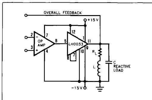
Figure 5. Isolation Buffer
