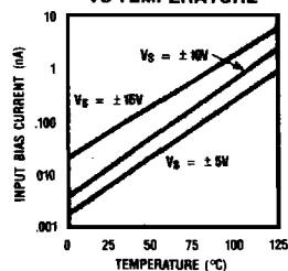
LH0033 INPUT BIAS CURRENT VS TEMPERATURE
