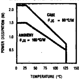
LH0033 POWER DISSIPATION
