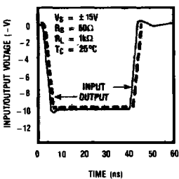
LH0033 NEGATIVE PULSE RESPONSE
