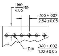
RECOMMENDED PC BOARD LAYOUT
