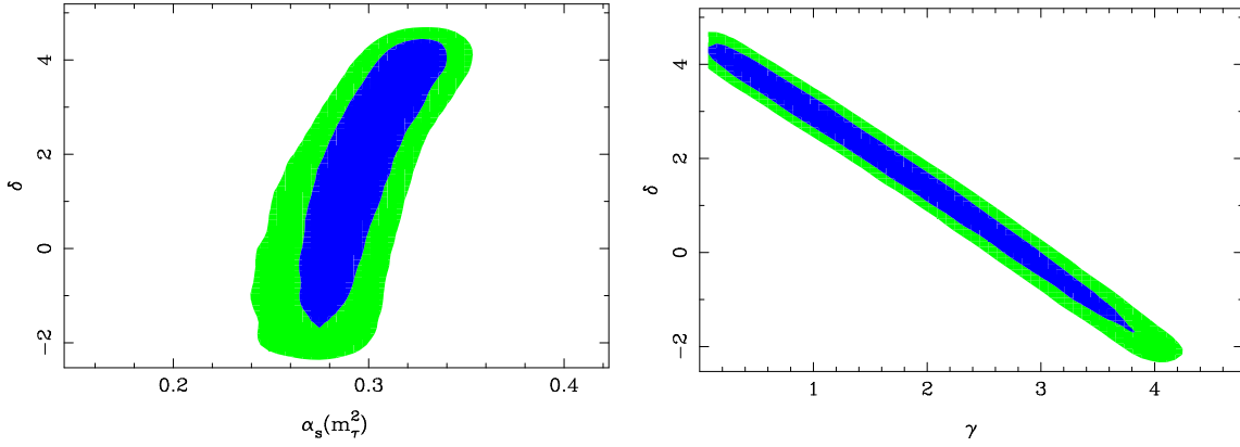
FIG. 2: Two-dimensional contour plots showing \alpha_s(m_\tau^2) versus \delta_V and \gamma_V versus \delta_V . Left panel: projection onto \alpha_s(m_\tau^2) - \delta_V plane. Right panel: projection onto \gamma_V - \delta_V plane. V channel, s_{min} = 1.5 \text{ GeV}^2 . Blue (darker) areas and green (lighter) areas contain 68%, respectively, 95% of the distribution.
