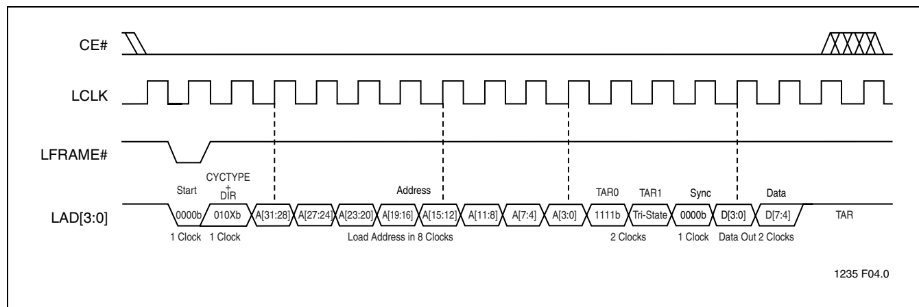
FIGURE 5: LPC Read Cycle Waveform
