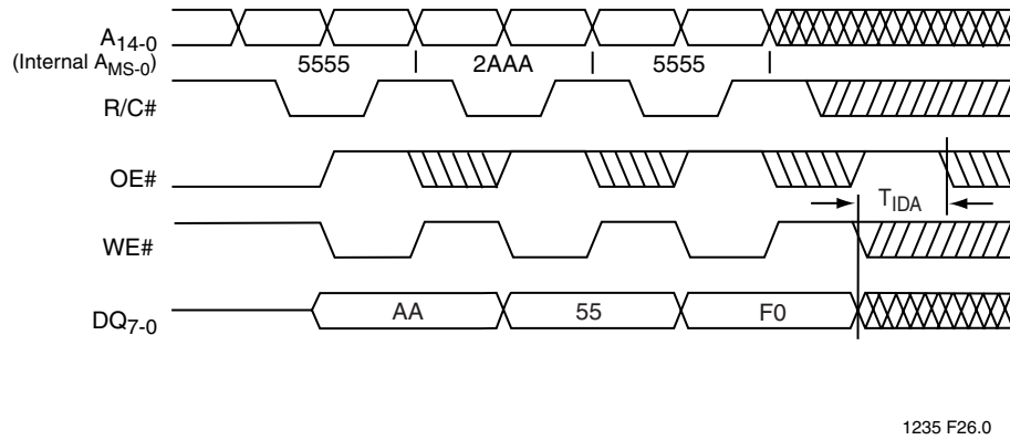
FIGURE 27: Software ID Exit (PP Mode)
