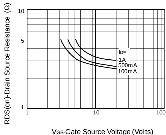
On-resistance v gate-source voltage
