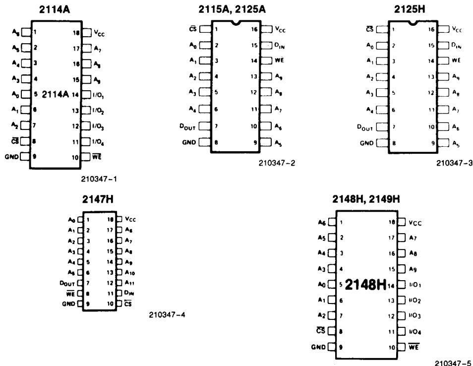
Pin Configuration
