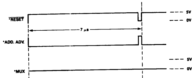
Figure 2. 2115, 2125 Burn-In Configuration
