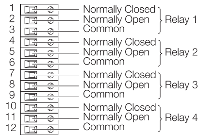
Four-Relay Output Module
