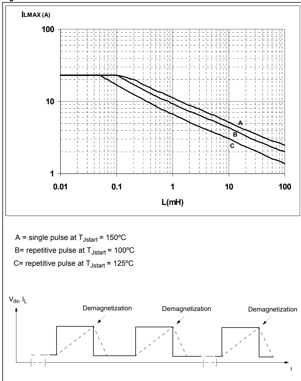
Figure 26. Maximum turn-off current versus load inductance
