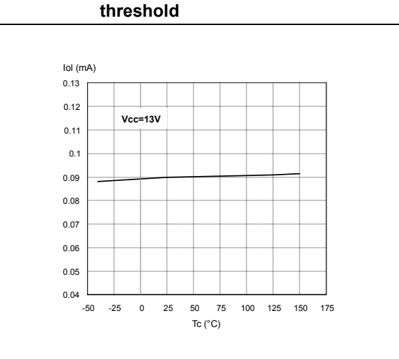
Figure 22. Openload on-state detection threshold
