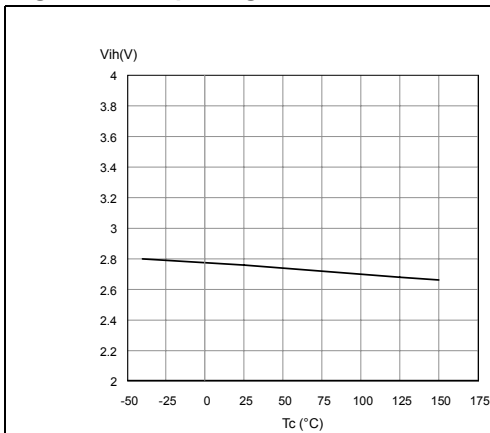
Figure 15. Input high level
