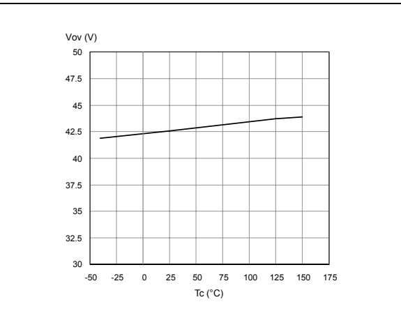
Figure 11. Overvoltage shutdown
