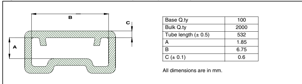
Figure 40. PowerSSO-12™ tube shipment (no suffix)
