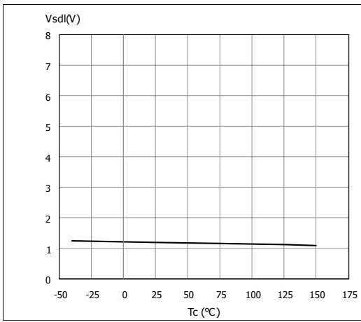
Figure 26. Low level STAT_DIS voltage
