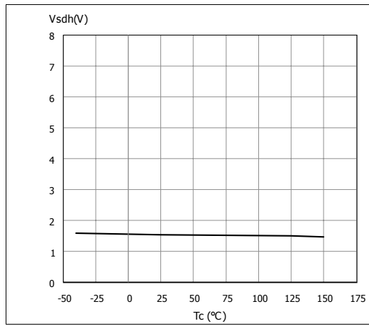
Figure 25. High level STAT_DIS voltage
