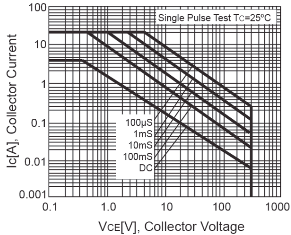
Figure 7. Safety Operation Area
