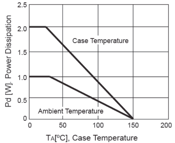
Figure 8. Derating Curve
