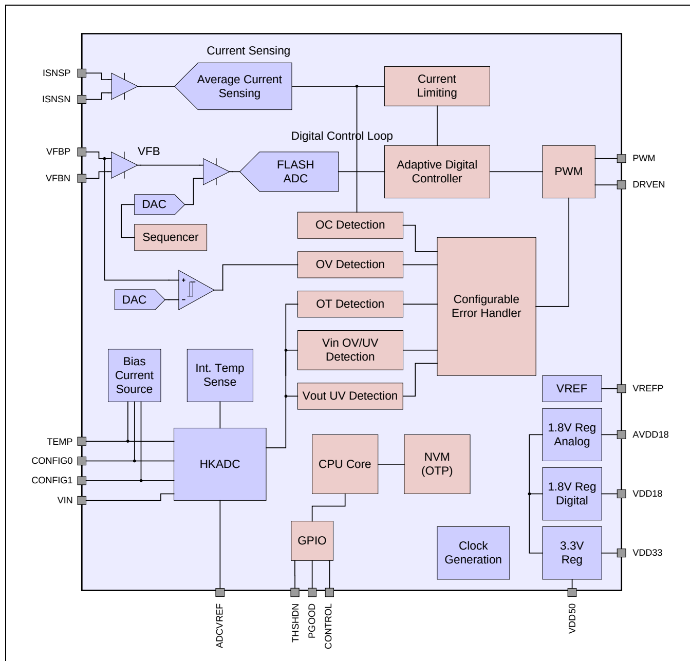
Figure 2.2 Block Diagram
