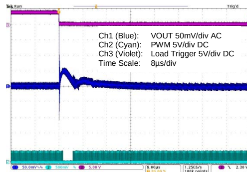
Figure 5.34 ZSPM1502 with Comp2; 15A to 5A Load Step; and Max. Capacitance
