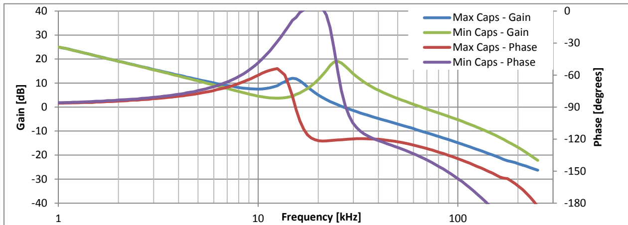
Figure 5.5 Open Loop Bode Plots for ZSPM1501 with Comp0
