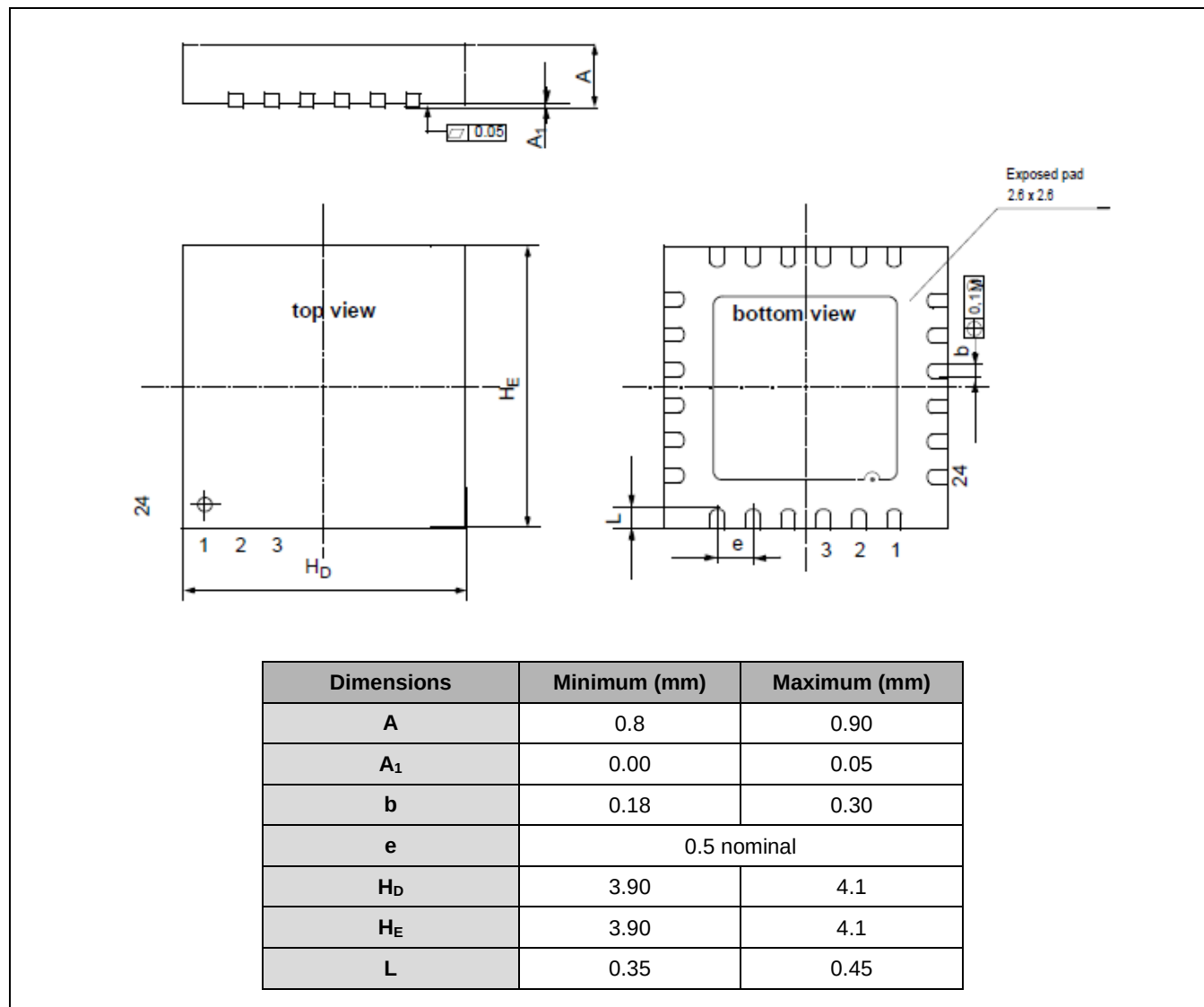
Figure 6.1 24-Pin QFN Package Drawing
