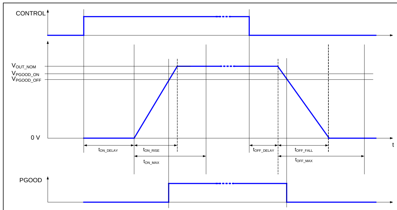
Figure 3.2 Power Sequencing
