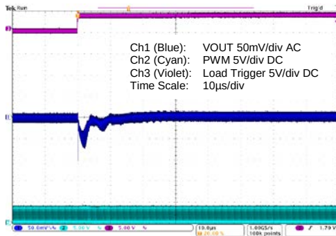
Figure 5.73 ZSPM1504 with Comp2; 5A to 15A Load Step; and Max. Capacitance
