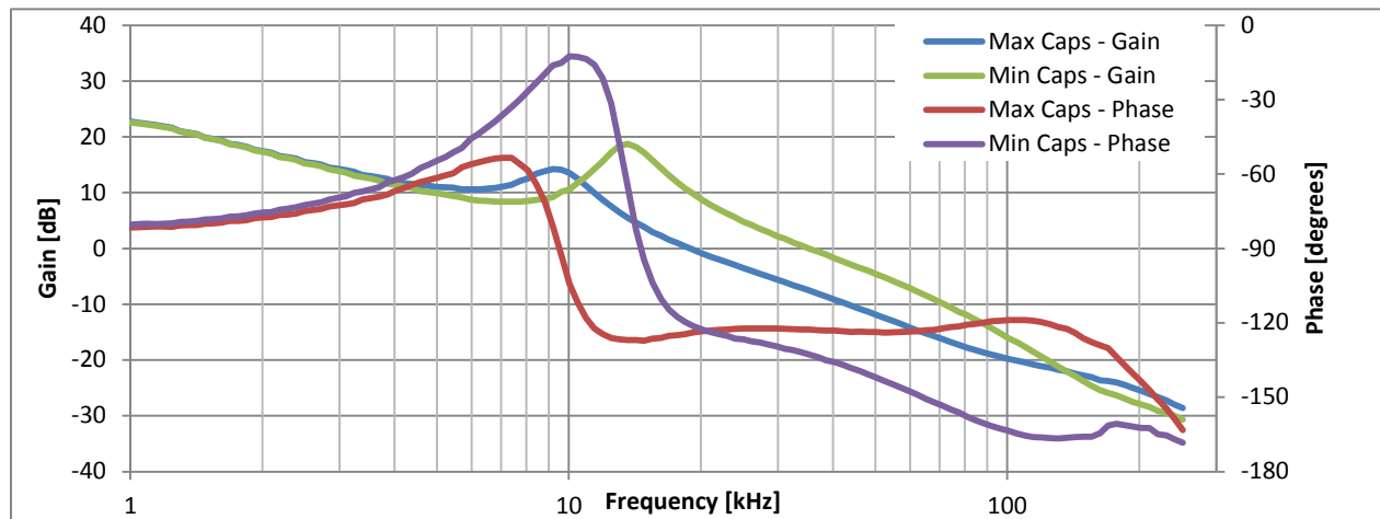
Figure 5.90 Open Loop Bode Plots for ZSPM1505 with Comp1
