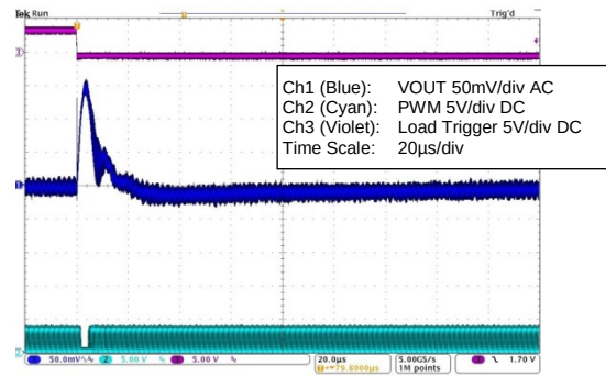
Figure 5.164 ZSPM1509 with Comp0; 8A to 3A Load Step; and Max. Capacitance
