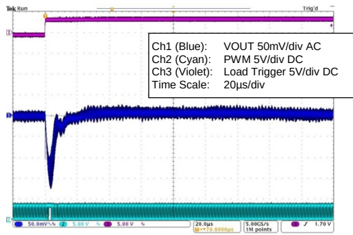
Figure 5.163 ZSPM1509 with Comp0; 3A to 8A Load Step; and Max. Capacitance
