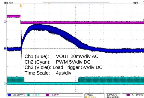
Figure 5.199 ZSPM1511 with Comp3; 15A to 5A Load Step; and Max. Capacitance
