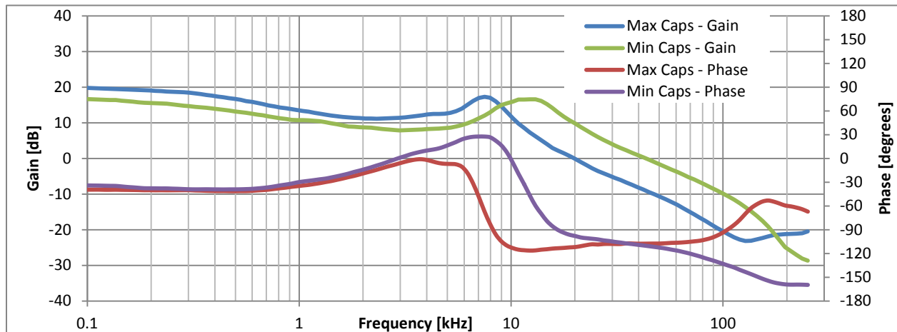
Figure 5.165 Open Loop Bode Plots for ZSPM1509 with Comp0
