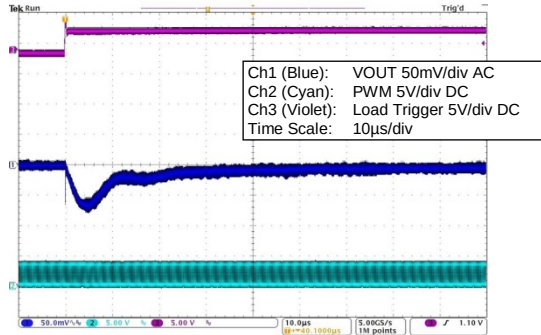
Figure 5.148 ZSPM1508 with Comp1; 5A to 10A Load Step; and Max. Capacitance
