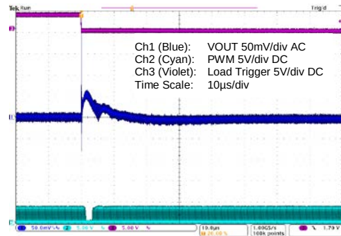
Figure 5.74 ZSPM1504 with Comp2; 15A to 5A Load Step; and Max. Capacitance
