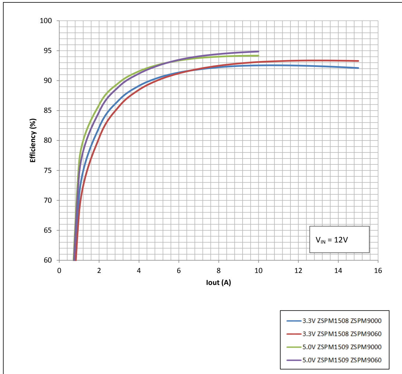
Figure 5.243 Typical Efficiency Curves: ZSPM9000 and ZSPM9060 DrMOS with ZSPM1508 and ZSPM1509
