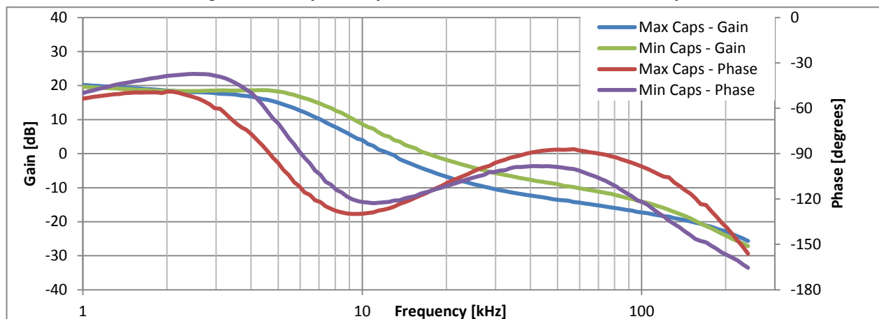
Figure 5.75 Open Loop Bode Plots for ZSPM1504 with Comp2
