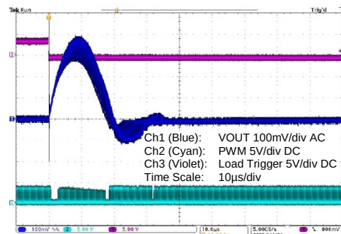
Figure 5.224 ZSPM1513 with Comp0; 15A to 5A Load Step; and Max. Capacitance
