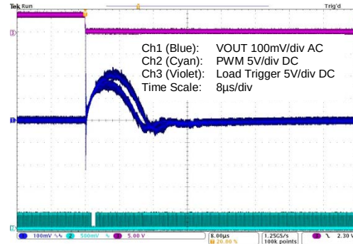
Figure 5.24 ZSPM1502 with Comp0; 15A to 5A Load Step; and Max. Capacitance
