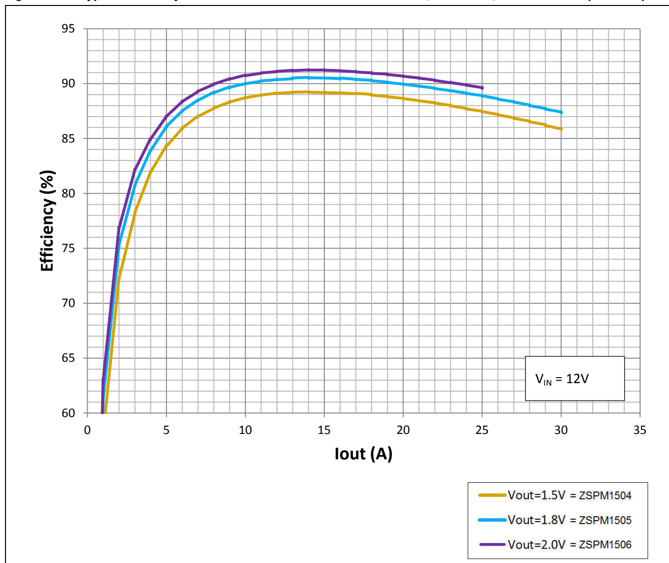
Figure 5.242 Typical Efficiency Curves: ZSPM9000 DrMOS with ZSPM1504, ZSPM1505, and ZSPM1506 ( V_{IN} = 12V )
