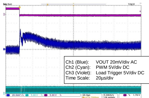
Figure 5.174 ZSPM1509 with Comp2; 8A to 3A Load Step; and Max. Capacitance
