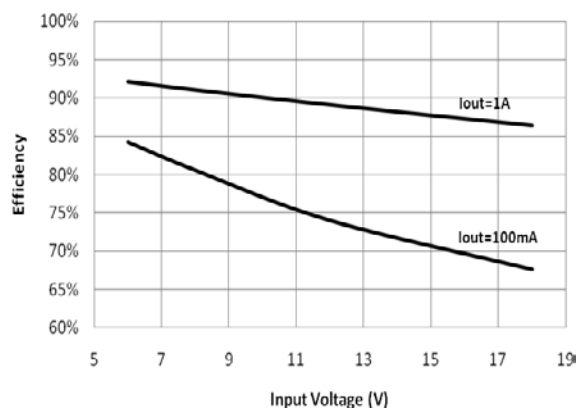
Figure 2.12 Efficiency vs. Input Voltage ( V_{OUT} = 3.3V )
