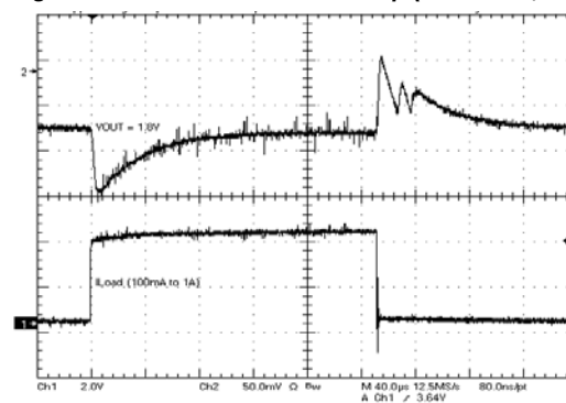
Figure 2.2 100mA to 1A Load Step ( V_{CC}=12\text{V} , V_{OUT}=1.8\text{V} )
