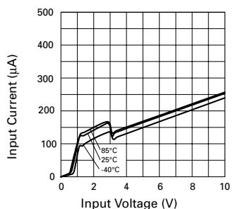
Input Current v Input Voltage
