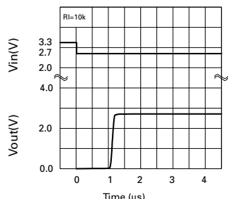
Reset Delay Time
