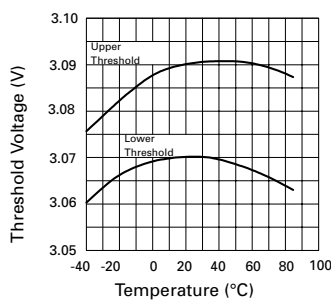
Threshold Voltage v Temperature
