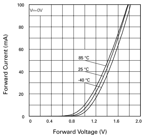
Clamp Diode Forward Current vs. Voltage
