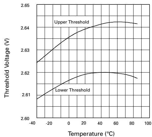
Threshold Voltage vs. Temperature
