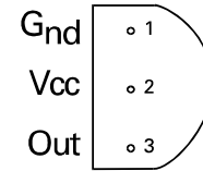
TO92 Package Suffix – C
