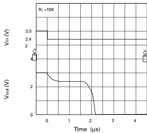
Reset Delay Time
