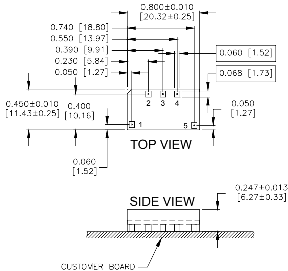
YM12S Pinout (Surface Mount)
