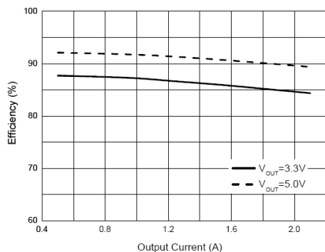
Fig. 4: Efficiency vs. Output Current
