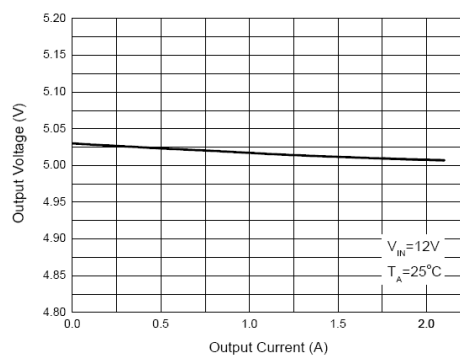
Fig. 13: Output Voltage vs. Output Current
