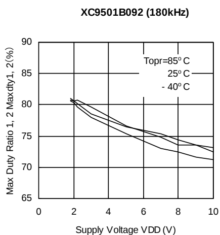
(12) Maximum Duty Ratio1, 2 vs. Supply Voltage
