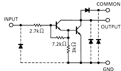
TD62003PAPG/AFG
