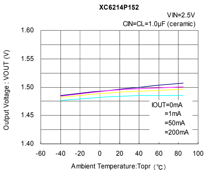
(5) Output Voltage vs. Ambient Temperature
