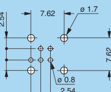
P19 - EPG-EXG (0B/1B.305) Screw mount
