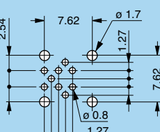
P19 - EPG-EXG (0B.309) Screw mount
