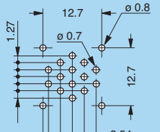
P20 - EPG.1B.314 Solder mount
