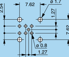
P19 - EPG-EXG (0B/1B.307) Screw mount
