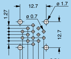
P20 - EPG.1B.314 Screw mount
