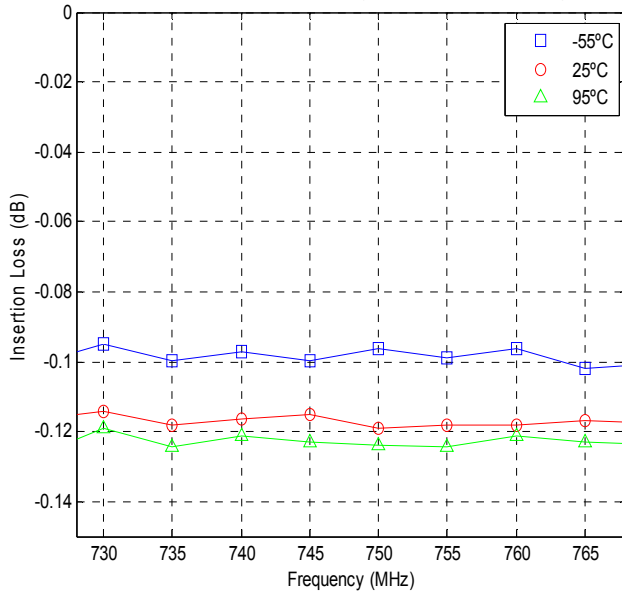
Insertion Loss for X3DC07E2S (Maximum Power Condition)
