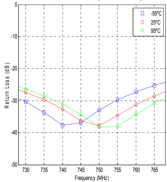
Return Loss for X3DC07E2S (Low Power Condition)
