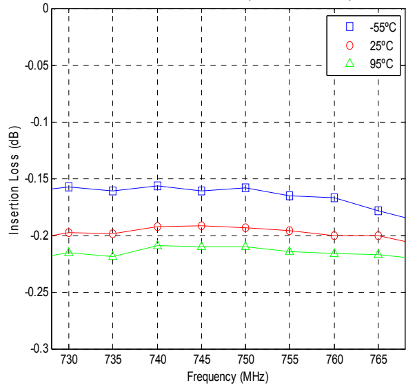
Insertion Loss for X3DC07E2S (Low Power Condition)
