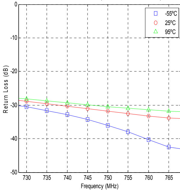
Return Loss for X3DC07E2S (Maximum Power Condition)
